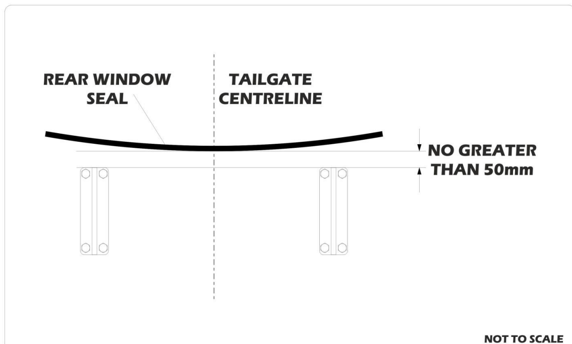
Figure 2: Series Approved Wing Mounting Position
